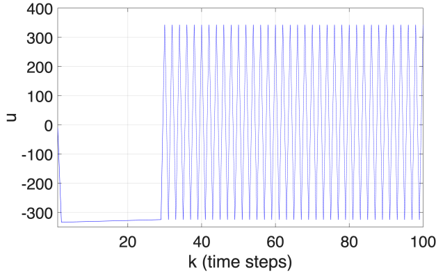
(c) MATLAB, zoomed k \in [0, 100] .
