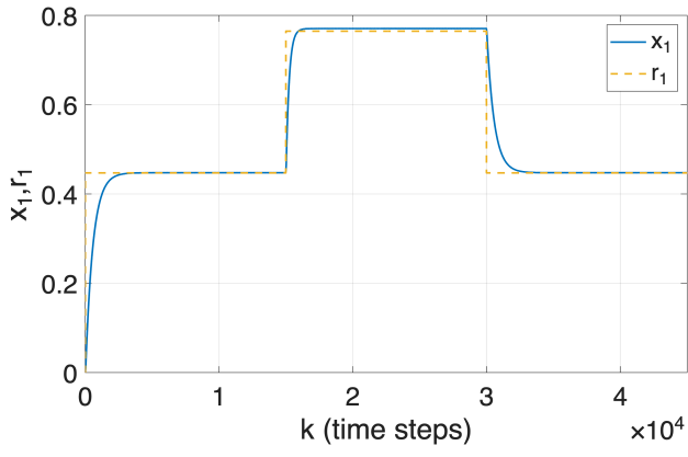
(a) MATLAB, conversion x_1 .
