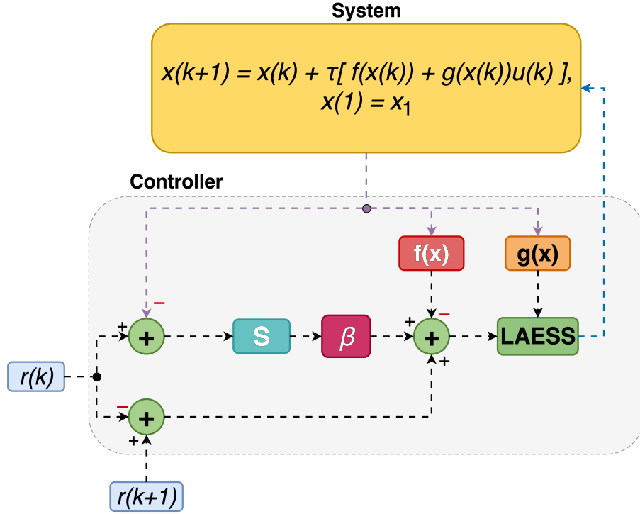
Figure 1: Functional block-diagram of the controlled nonlinear system.
